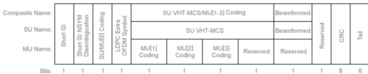
VHT-SIG-A2 Structure
